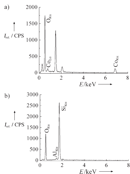
Figure 2. The surface EDS analysis results: a) \text{Co}/\text{Al}_2\text{O}_3 pellet; atomic ratio: Al 91.24%, Co 8.76%; b) after the hydrothermal synthesis; atomic ratio: Al 4.08%, Si 95.92%.
